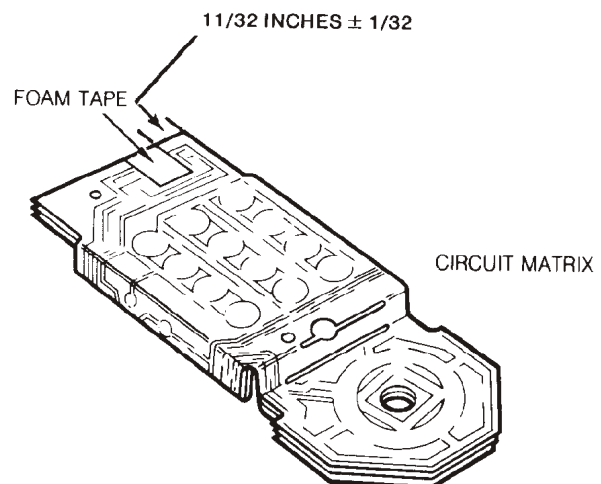
Figure 13 Foam Tape Replacement
