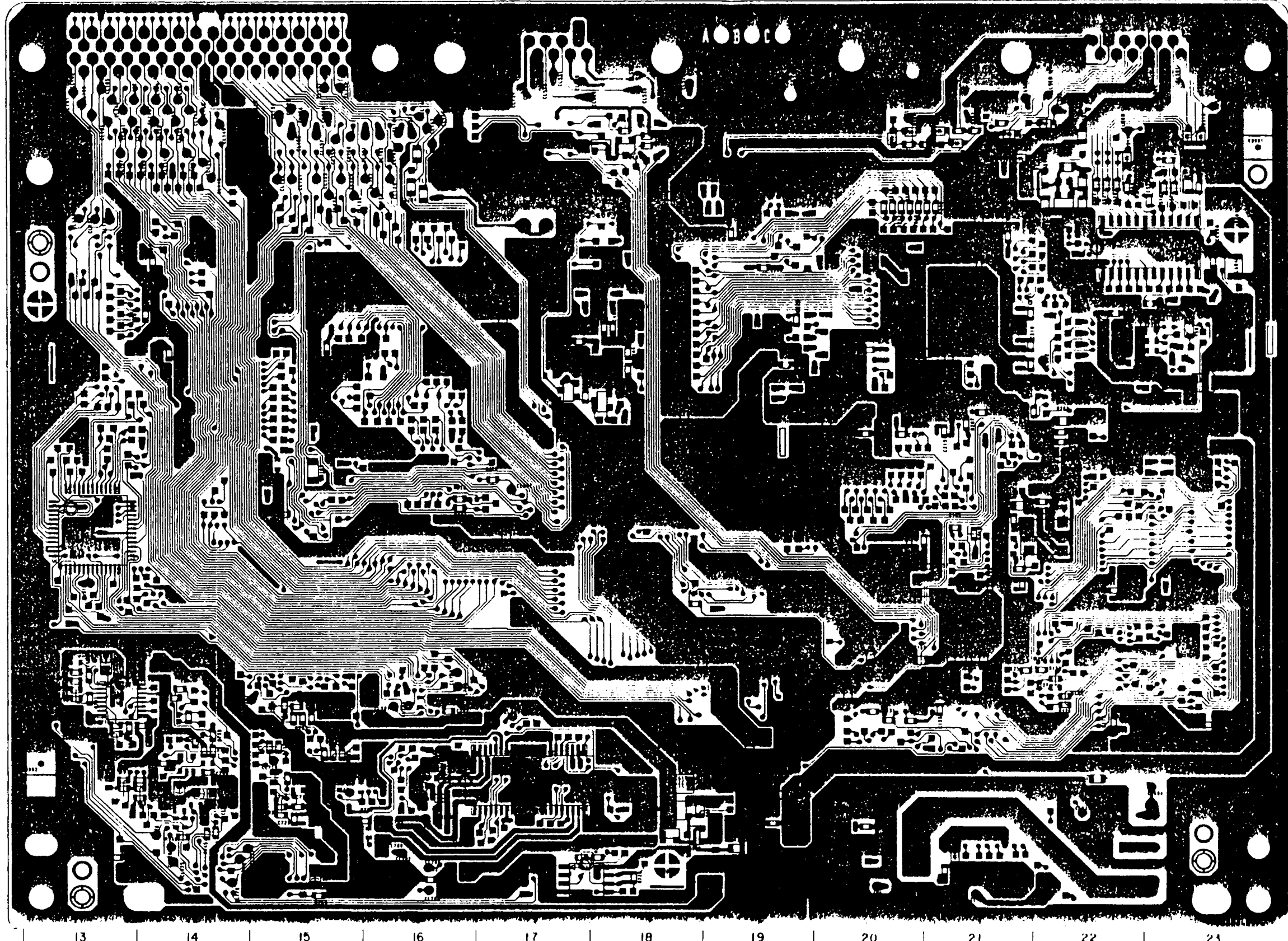
PU-18 BOARD (SIDE B)
