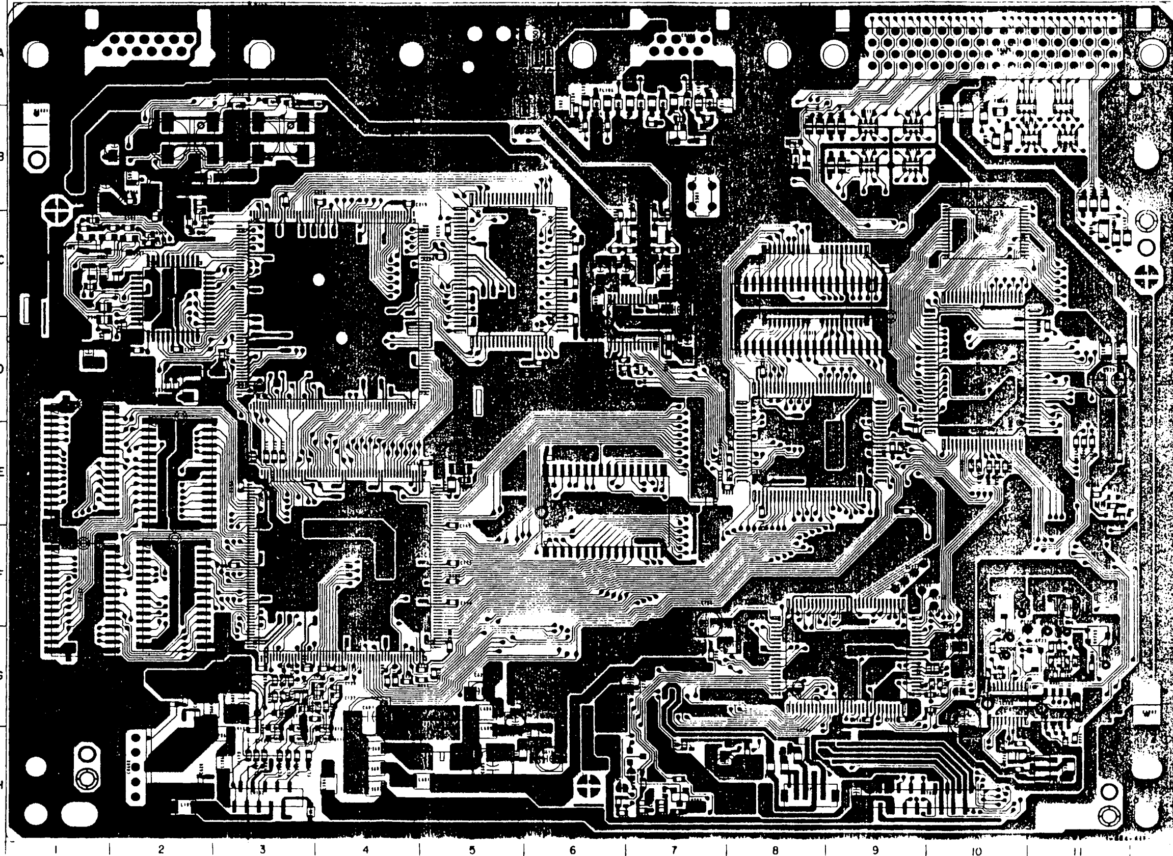
PU-18 BOARD (SIDE A)
